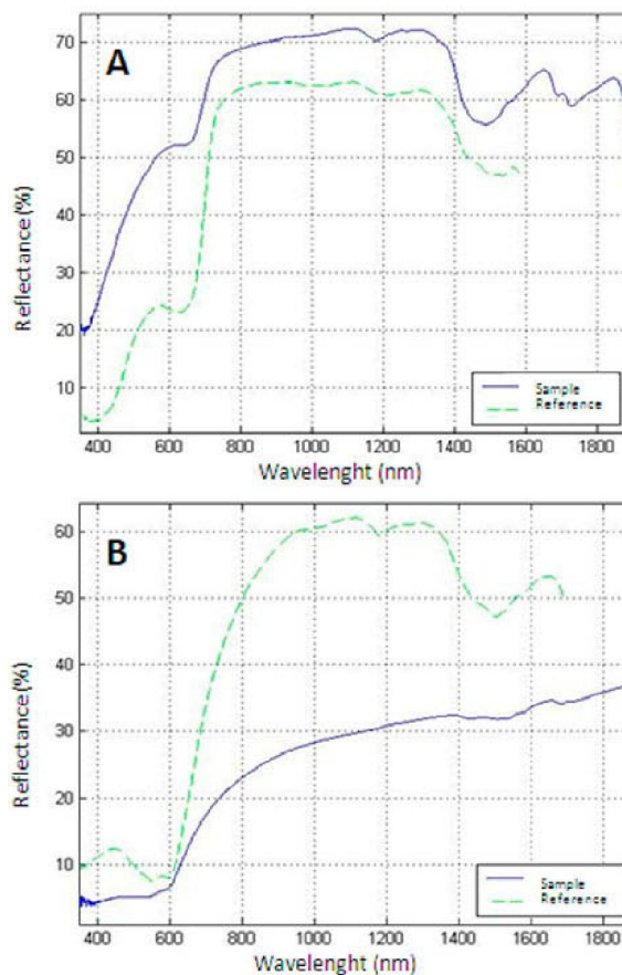
Figure 8: A: FORS analysis of the green border of the kikkō (blue line), compared to the one obtained by the analysis of a reference silk thread dyed with indigo + yellow safflower (green dotted line); B: FORS analysis of the purplish inner part of the kikkō (blue line), compared to the one obtained by the analysis of a reference silk thread dyed with alkanet (green dotted line).
