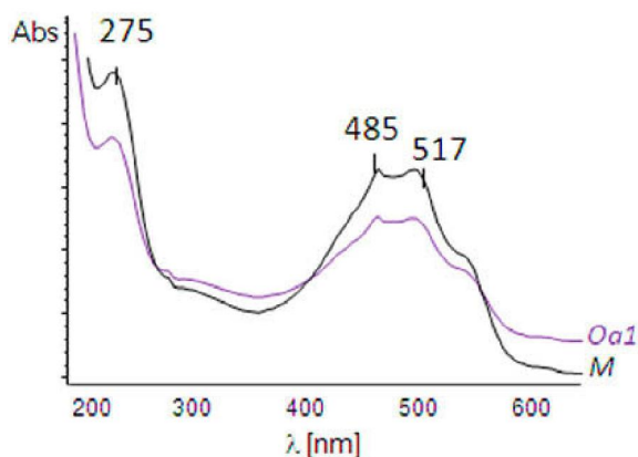
Figure 10: DAD spectra obtained for the peaks at 18 minutes for the chromatograms shown in Figure 9, assigned to hydroxy-naphthoquinones.
