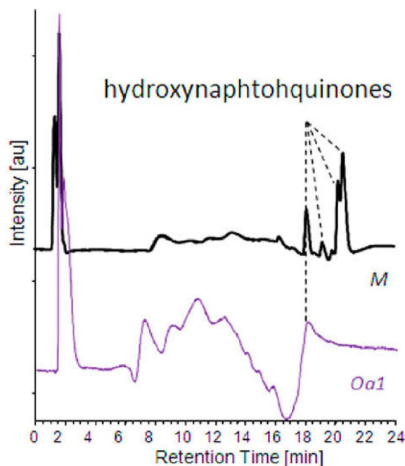
Figure 9: HPLC-DAD chromatograms at 490 nm of the DMSO extract of the purplish thread in the kikkō (sample Oa1) and of the DMSO extract of the ex-novo fabric dyed with murasaki (M).
