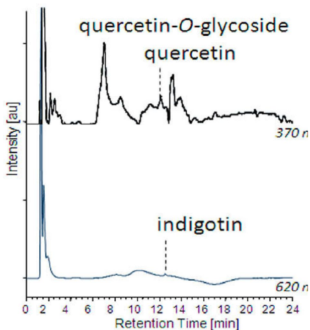
Figure 6: HPLC-DAD chromatograms of the extracts of the weft of the silk damask (sample D5): DMSO extract, at 620 nm (blue line) and extract after mild methanolysis, at 370 nm (black line).
