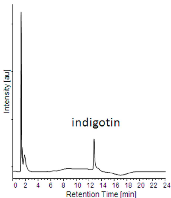
Figure 5: HPLC-DAD chromatogram of the DMSO extract of the warp of the silk damask, at 620 nm (sample D2).
